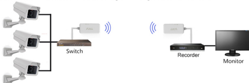
Solution Three Camera 1,2,3---Switch-Bridge Bridge---Recorder---Monitor
